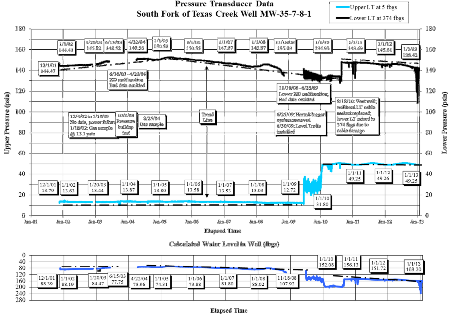
Figure 2-5 Pressure Transducer Data South Fork of Texas Creek Well MW-35-7-8-1
