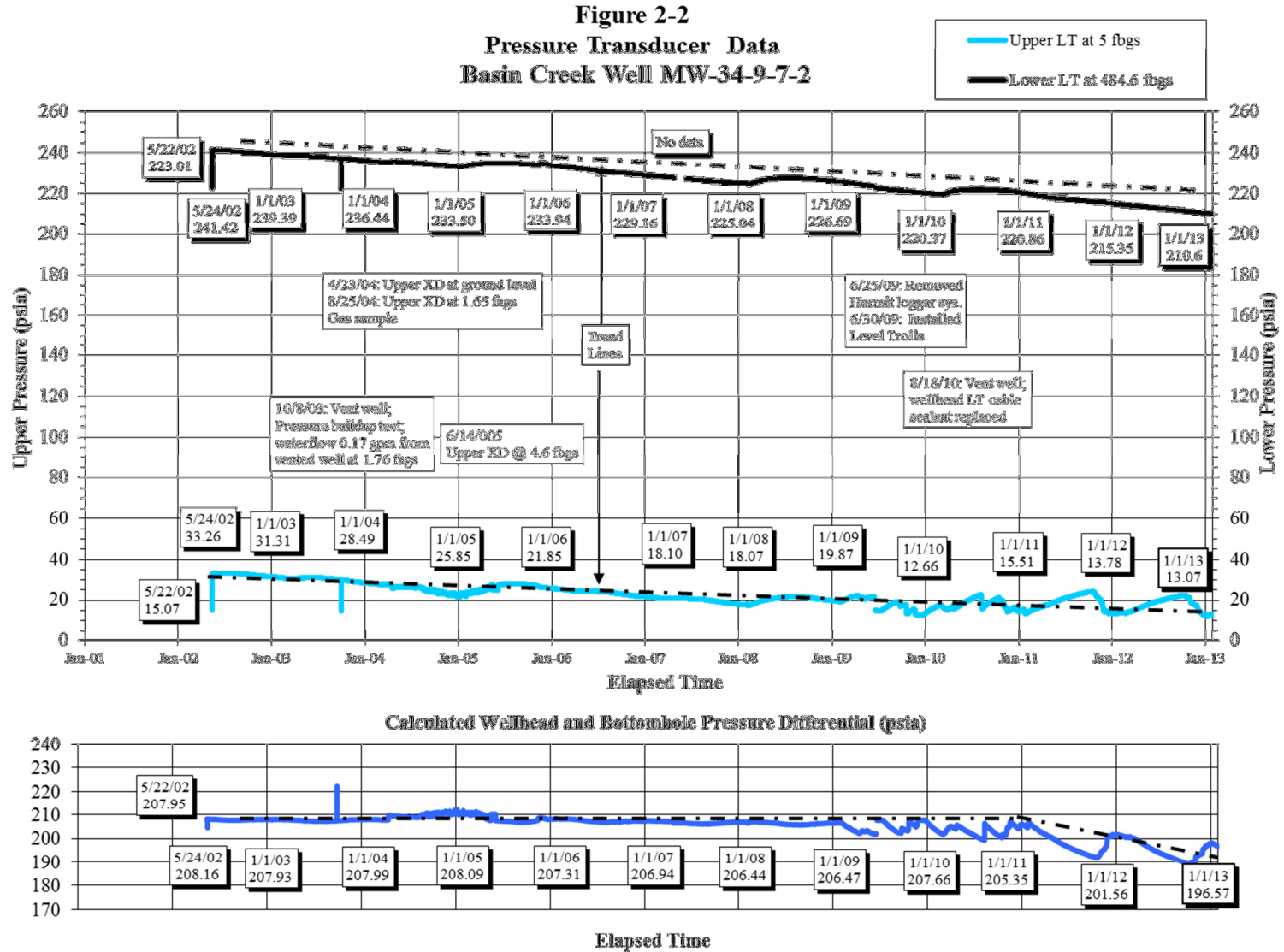
Figure 2-2 Pressure Transducer Data Basin Creek Well MW-34-9-7-2
