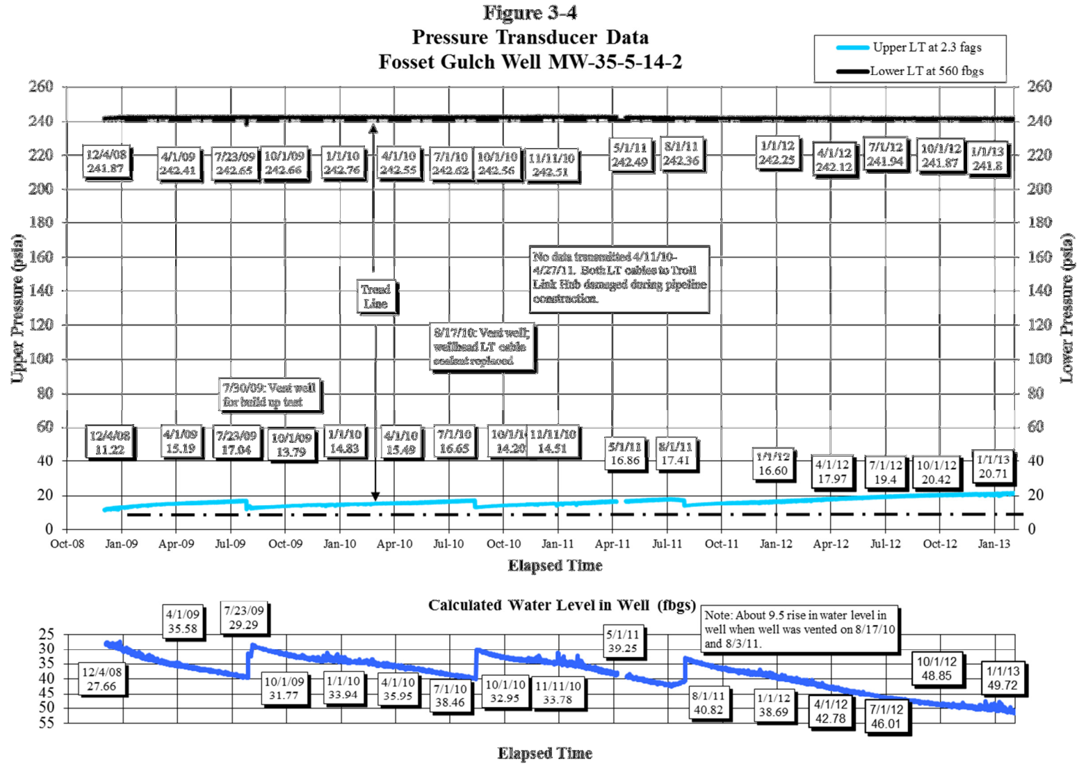
Figure 3-4 Pressure Transducer Data Fosset Gulch Well MW-35-5-14-2
