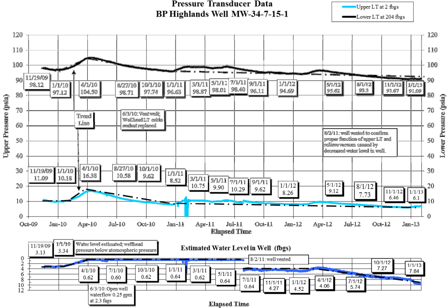
Figure 2-7 Pressure Transducer Data BP Highlands Well MW-34-7-15-1
