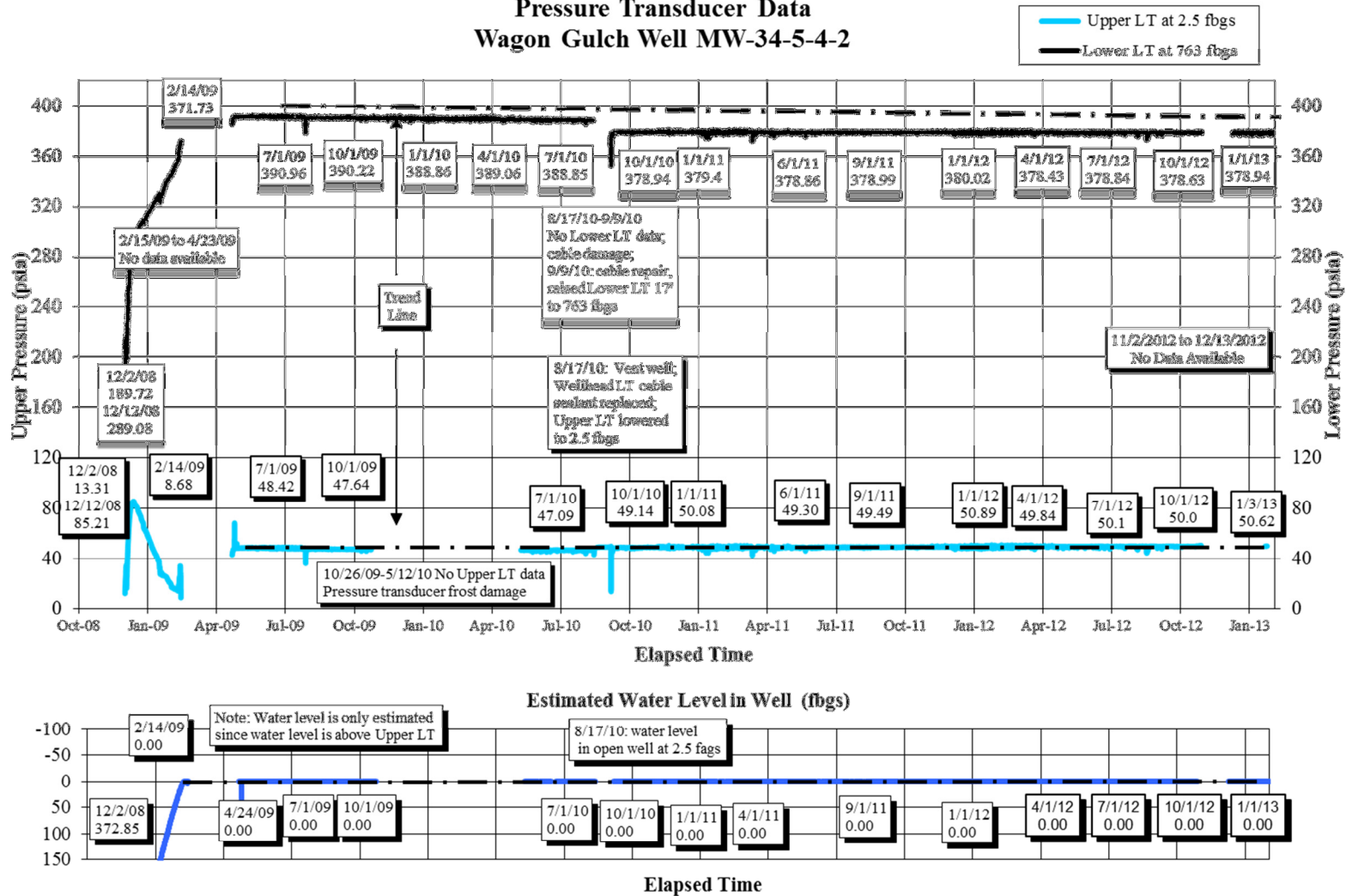
Figure 3-2 Pressure Transducer Data Wagon Gulch Well MW-34-5-4-2
