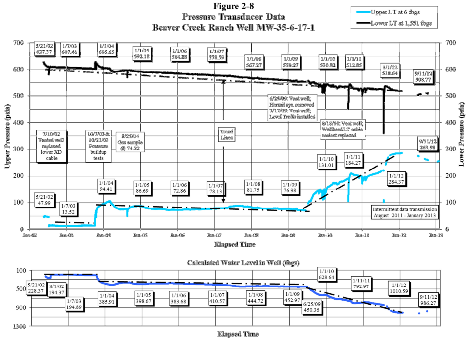
Figure 2-8 Pressure Transducer Data Beaver Creek Ranch Well MW-35-6-17-1
